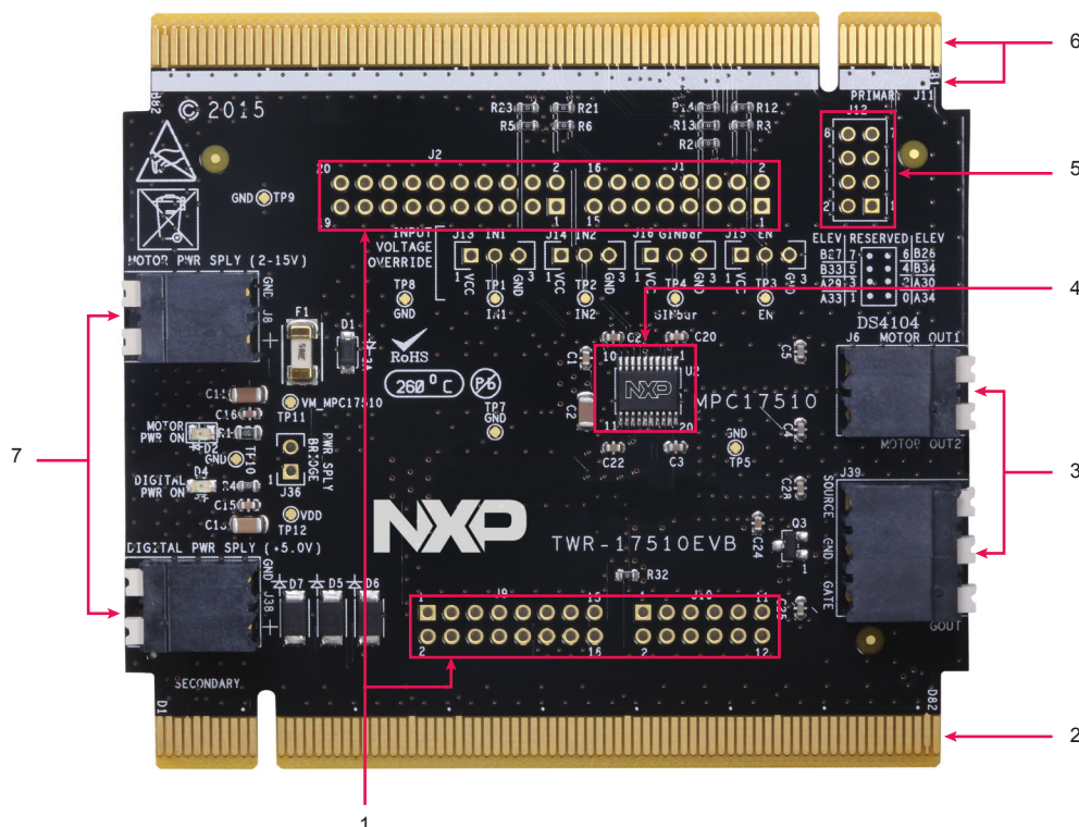
Figure 3. Board description
