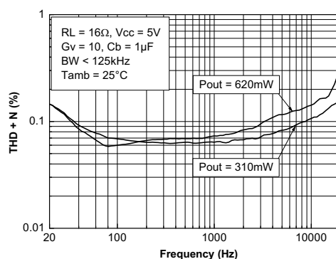
Figure 84. THD + N vs frequency (Vcc=5 V)
