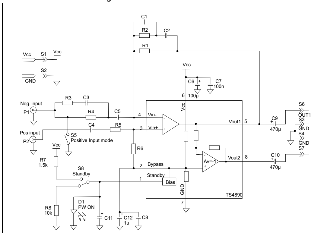
Figure 105. Demoboard schematic
