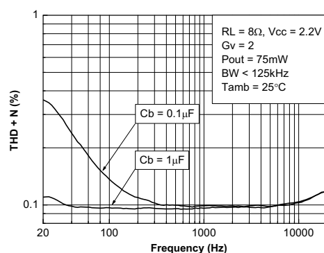
Figure 82. THD + N vs frequency (Vcc=2.2 V)
