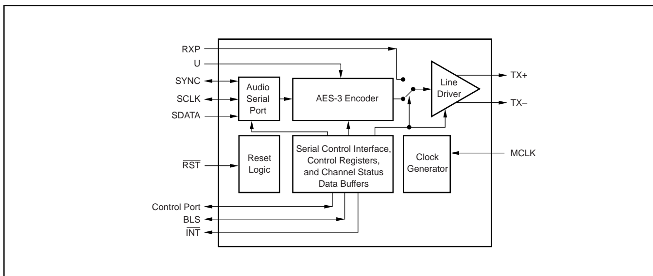
FIGURE 1. Software Mode Block Diagram.
