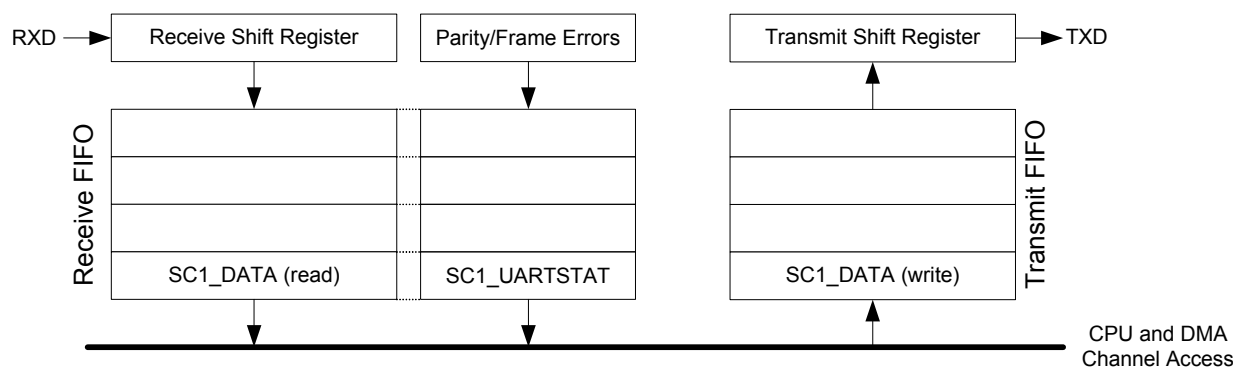
Figure 8.3. UART FIFOs
