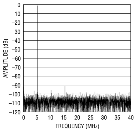
8192 Point FFT, f_{IN} = 5\text{MHz} , -1dB, 2V Range, 80Msps
