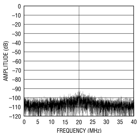
8192 Point FFT, f_{IN} = 140\text{MHz} , -1dB, 2V Range, 80Msps
