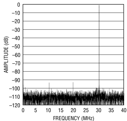
8192 Point FFT, f_{IN} = 30\text{MHz} , -1dB, 2V Range, 80Msps
