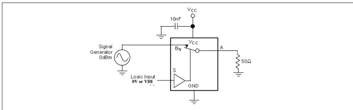
Figure 9. Bandwidth
