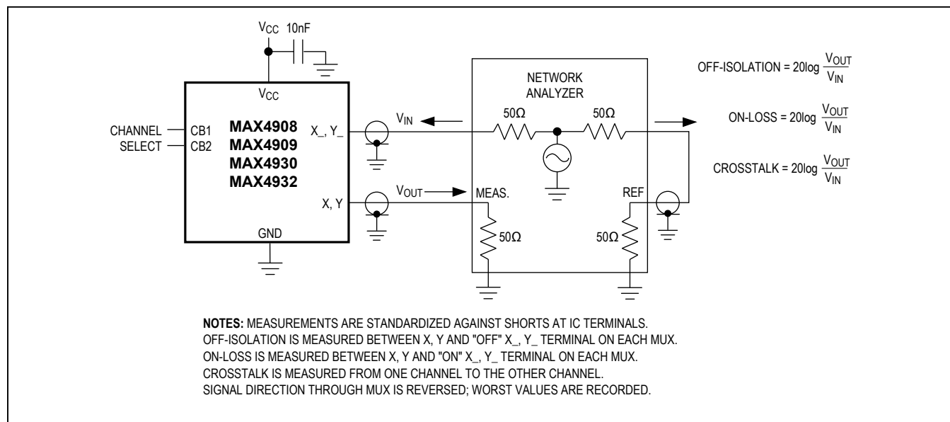
Figure 5. On-Loss, Off-Isolation, and Crosstalk
