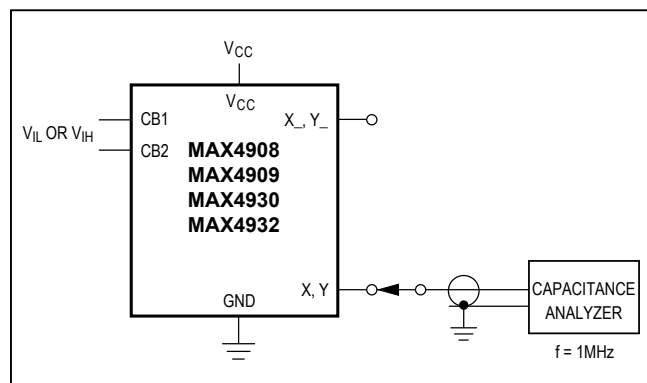
Figure 6. Channel Off/On-Capacitance
