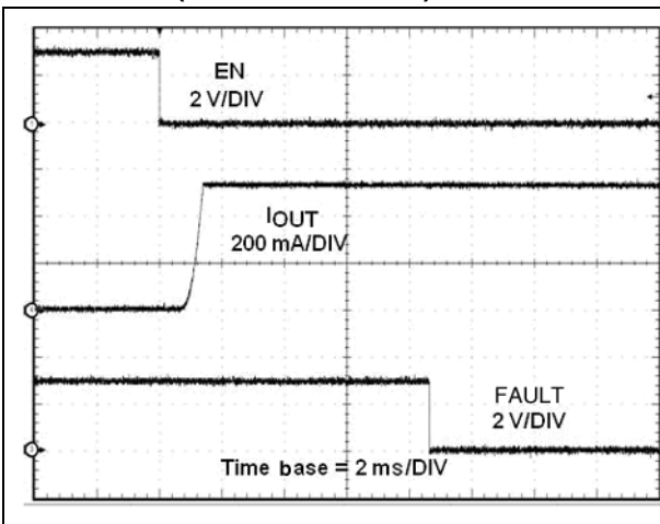
Figure 13. OC protection at V_{OUT} = 3.0\text{ V} (STMP52141/2151)
