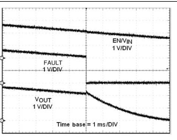
Figure 12. UVLO falling (STMP52141/2151)
