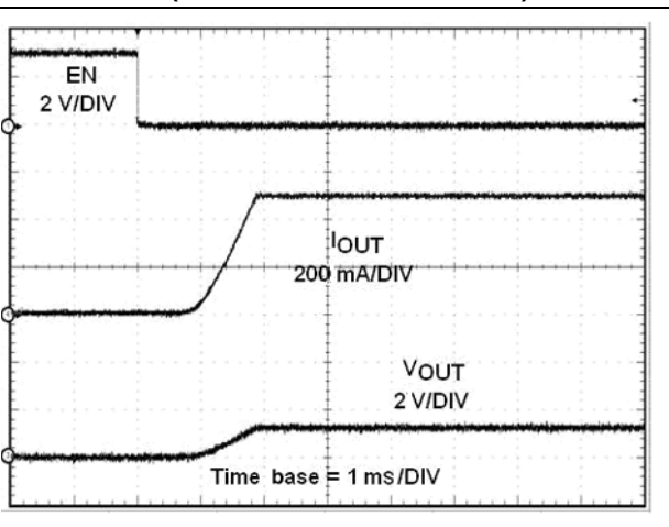
Figure 14. OC protection at V_{OUT} = 3.0\text{ V} (STMP52141/2151 - detail)
