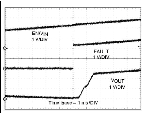
Figure 11. UVLO rising (STMP52141/2151)
