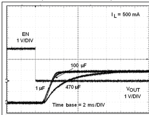
Figure 7. Voltage output turn-on delay time (STMPS2141/2151, 3 V)
