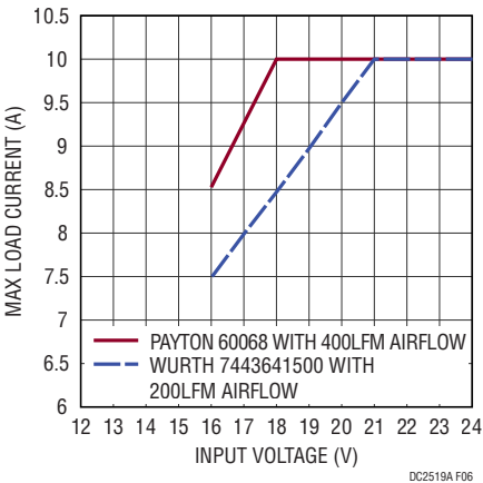
Figure 6. DC519A Output Current Derating vs Input Voltage
