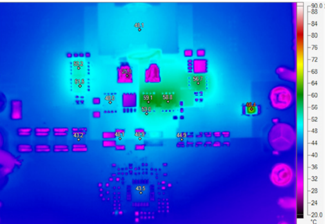
Figure 7. DC2519A Thermal Performance at 36V IN , 48V OUT , 10A Load Current with No Forced Airflow
