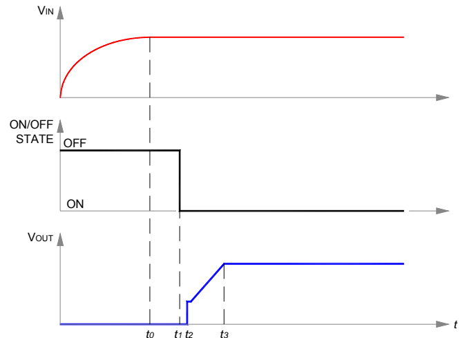
Fig. 8: Start-up scenario #2.
