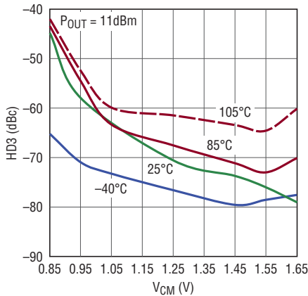
HD3 at 140MHz vs V_{CM} Over Temperature
