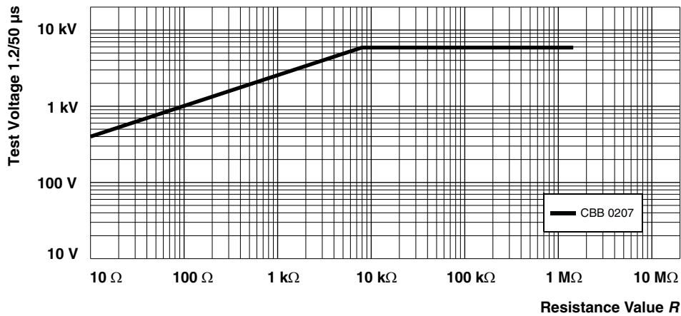
Pulse load rating in accordance with IEC 60115-1, 4.27; 1.2 μs/50 μs; 5 pulses at 12 s intervals; for permissible resistance change 0.5 %.
