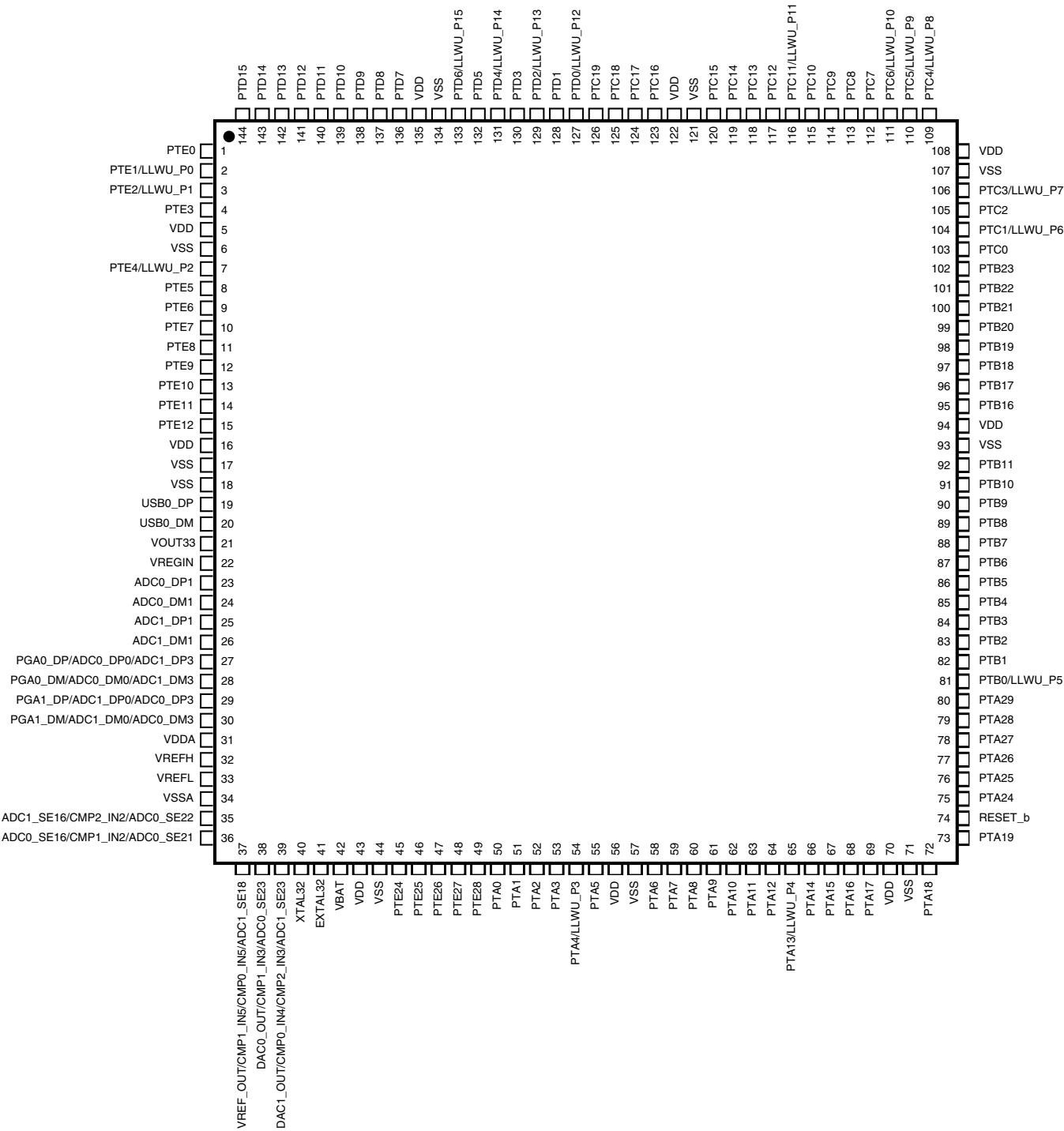
Figure 34. K60 144 LQFP Pinout Diagram
