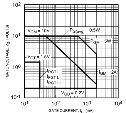
GATE CHARACTERISTICS (I, II, III)
