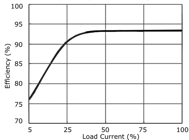
PDRA-240-24 Efficiency Curve (Efficiency vs. Load Current)
