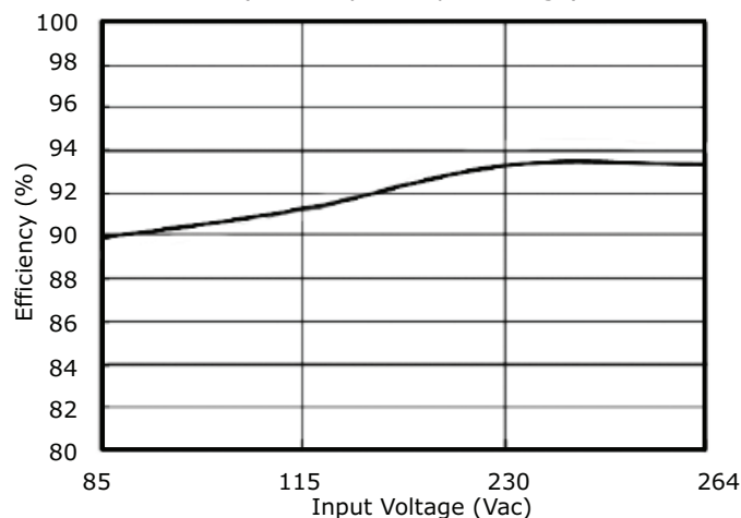
PDRA-240-24 Efficiency Curve (Efficiency vs. Input Voltage)
