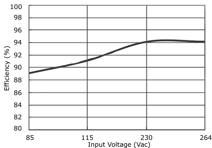
PDRA-240-48 Efficiency Curve (Efficiency vs. Input Voltage)
