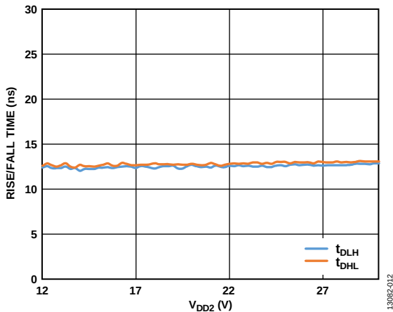
Figure 12. Typical Rise/Fall Time vs. V_{DD2} , V_{DD2} - V_{SS2} = 12\text{ V} , V_{DD1} = 5\text{ V} , 2\text{ nF} Load, R_G = 3.9\text{ }\Omega
