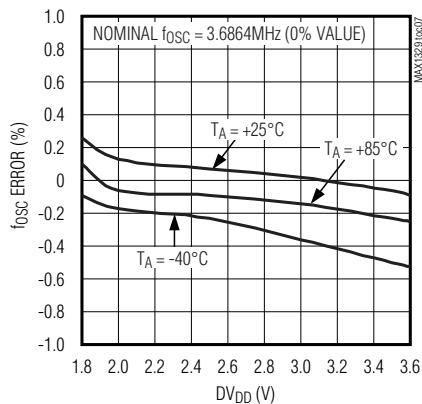
f_{OSC} ERROR vs. DIGITAL SUPPLY VOLTAGE
