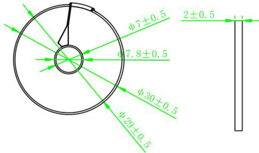
Antifreeze plate
