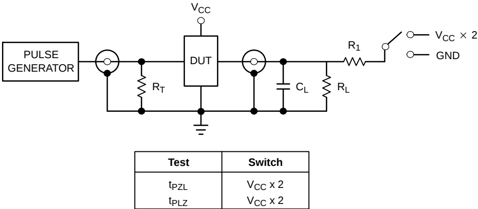
Figure 6. Test Circuit
