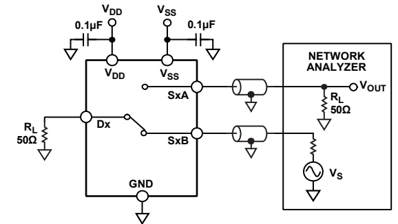
Figure 38. Bandwidth
