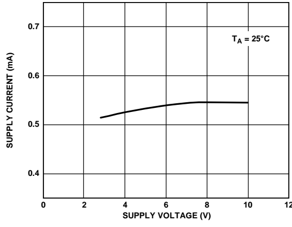
Figure 13. Supply Current/Amplifier vs. Supply Voltage
