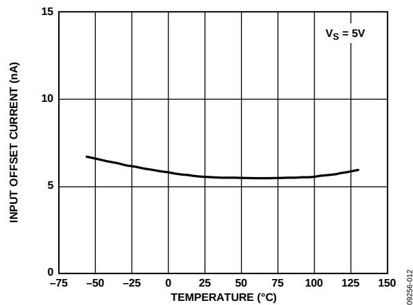
Figure 7. Input Offset Current vs. Temperature
