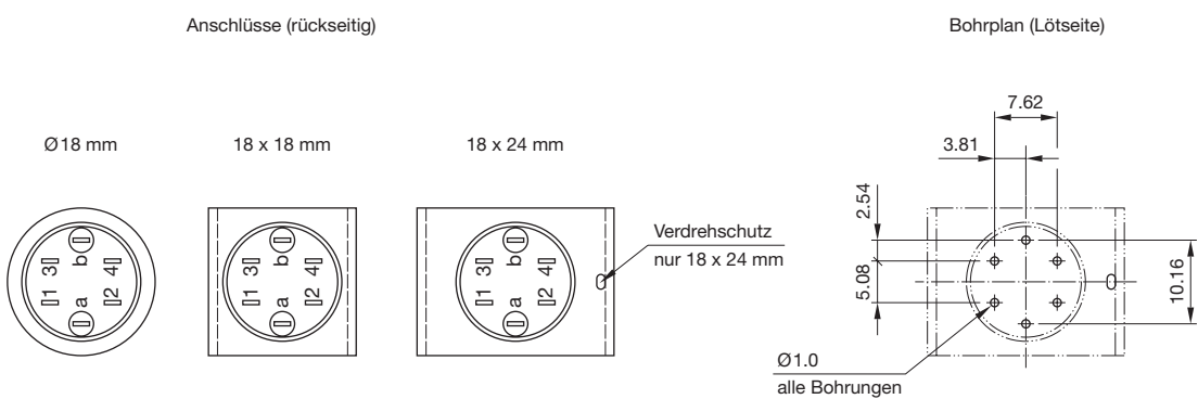
Component layout 4
