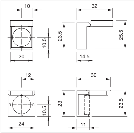
Dimensions [mm]
