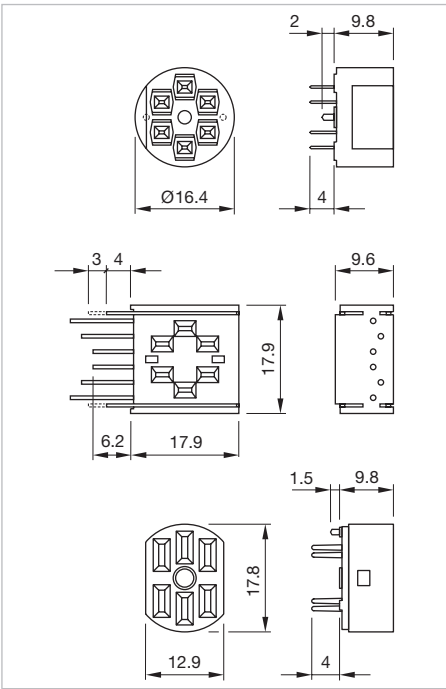
Dimensions [mm]
