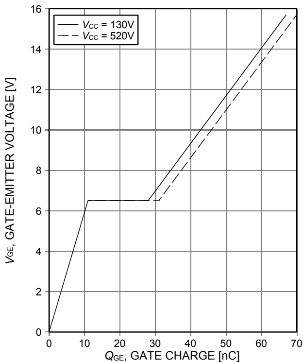
Figure 15. Typical gate charge ( I_C=30A )
