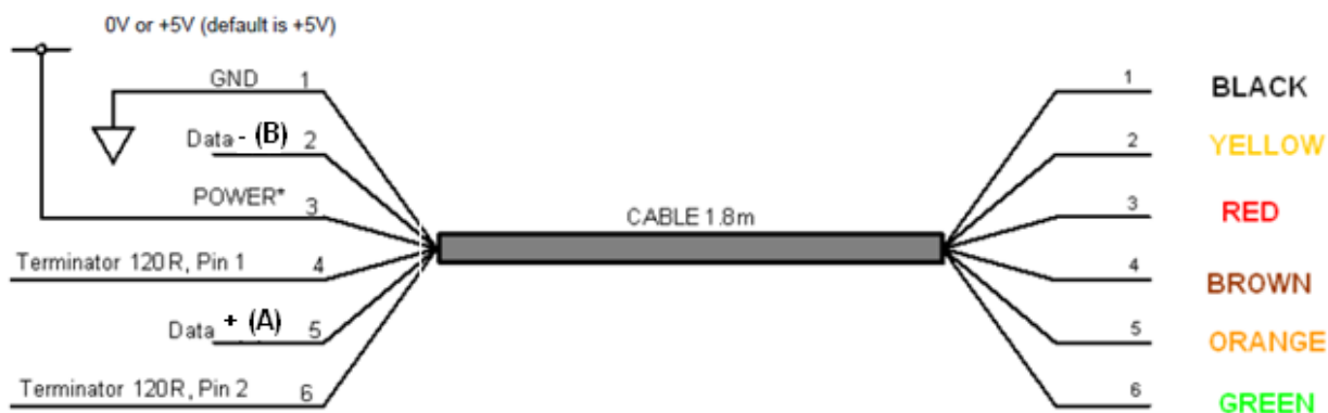
Figure 5.1 USB-RS485-WE Connections
