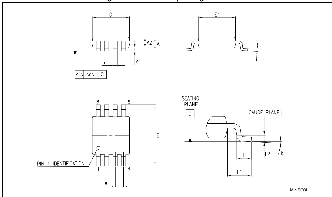
Figure 33. MiniSO8 package outline
