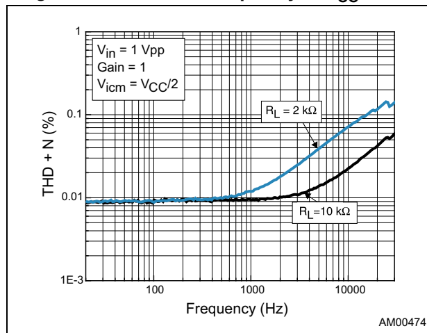
Figure 16. THD+N vs. frequency at V_{CC} = 2.7\text{ V}
