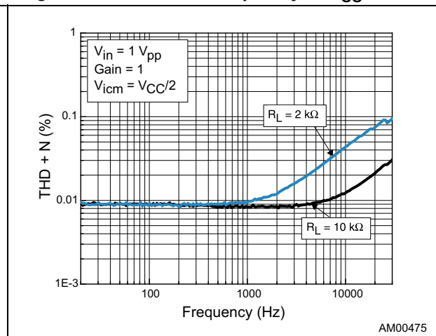
Figure 17. THD+N vs. frequency at V_{CC} = 5.5\text{ V}
