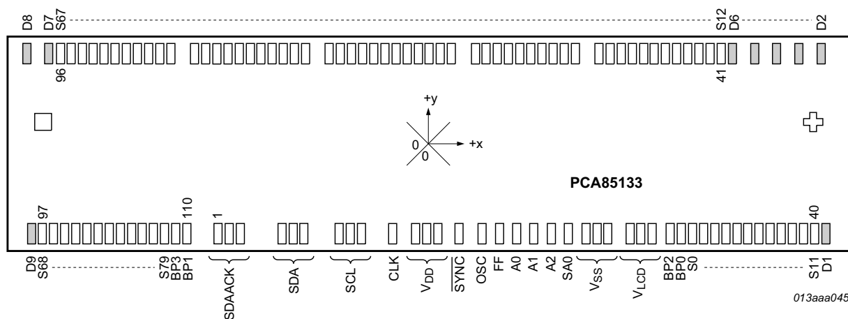
Fig 2. Pin configuration for PCA85133
