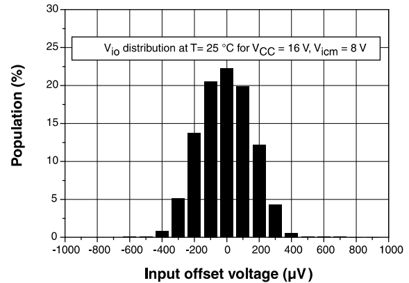
Figure 3: Input offset voltage distribution at V_{CC} = 16\text{ V} and V_{icm} = 8\text{ V}
