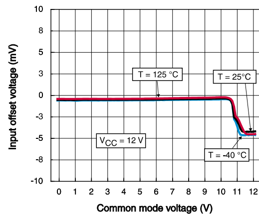
Figure 5: Input offset voltage vs. input common-mode voltage at V_{CC} = 12\text{ V}
