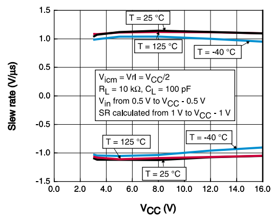
Figure 16: Slew rate vs. supply voltage
