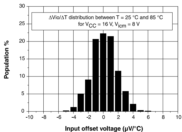
Figure 4: Input offset voltage temperature coefficient distribution at V_{CC} = 16\text{ V} , V_{icm} = 8\text{ V}
