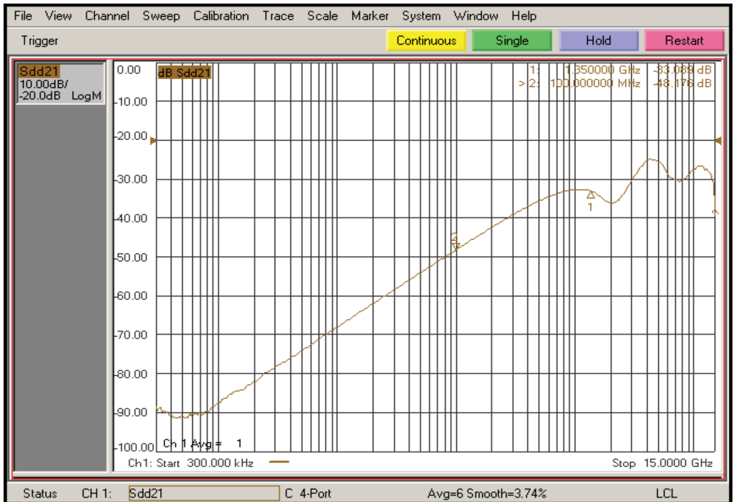
Fig 4. Xtalk
