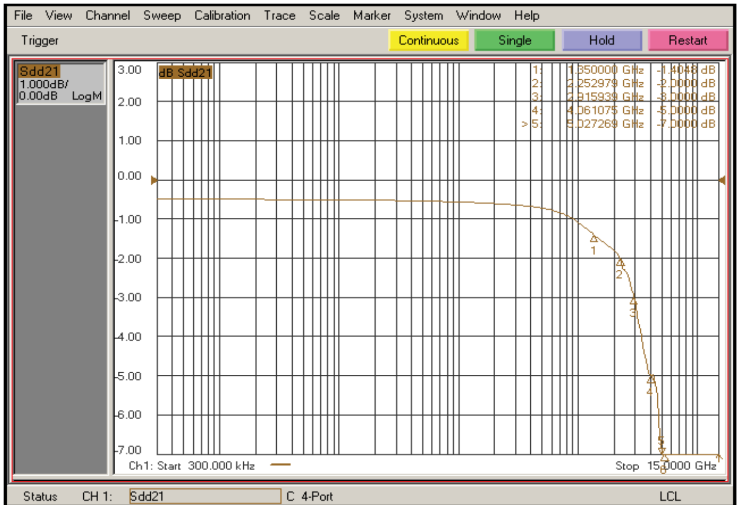
Fig 6. Insertion Loss
