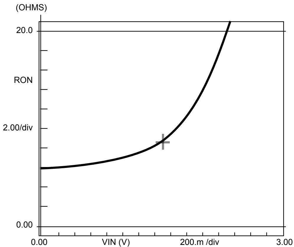
Fig 7. Ron Curve for High Speed Signal Path Only ( Dx\pm )
