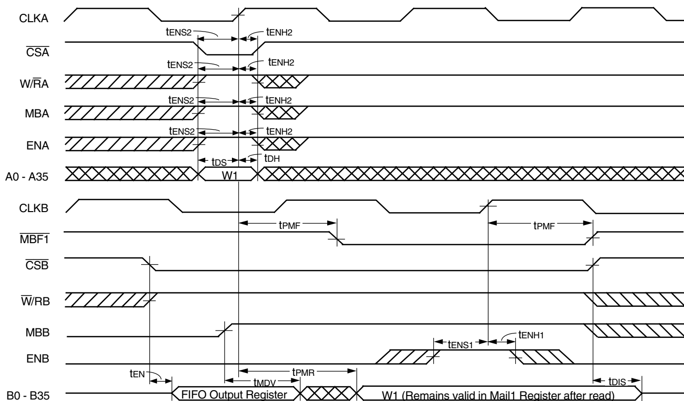
Figure 15. Timing for Mail1 Register and MBF1 Flag
