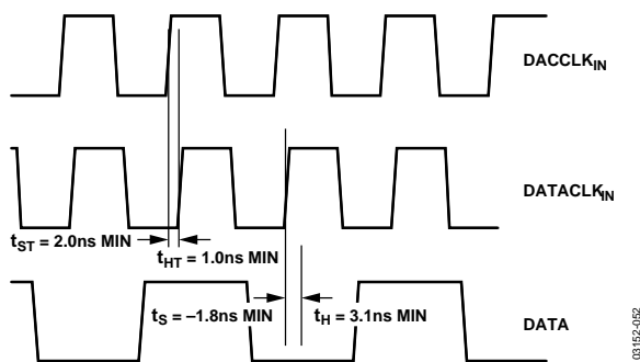
Figure 52. Low Setup and Hold Mode Timing, 1x Interpolation, DCLKPOL = 1
