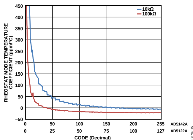
Figure 15. Rheostat Mode Temperature Coefficient ( (\Delta R_{WB}/R_{WB})/\Delta T \times 10^6 ) vs. Code
