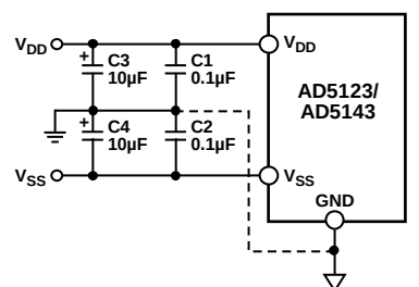
Figure 40. Power Supply Bypassing
